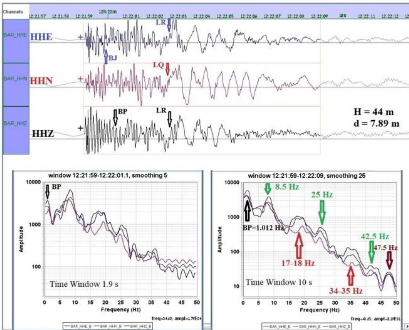
Figure 4: The positive (+) first motion of P-wave arrivals and the clear advent of a bubble pulse (BP) and a bubble jet (BJ) as well as Rayleigh (LR) and Love (LQ) waves in the time domain (upper) and spectral characteristic frequencies of 3-component spectra in the frequency domain (lower) at the BAR station comparing a short time window (1.9 s) with a long time window (10 s). The black arrows, red upward arrows, green downward arrows and a brown downward arrow indicate a bubble pulse frequency, reverberation frequencies from the bottom and reflection from the hull, and the reverberation frequency from the free surface, respectively
