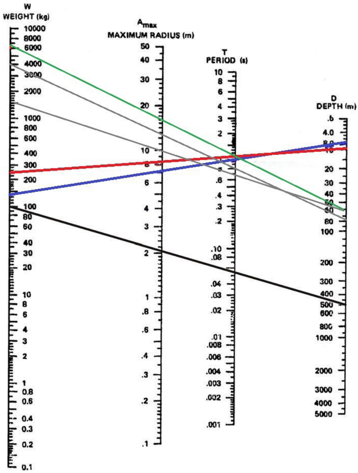
Figure 16: Nomograph of the first bubble pulse period, maximum bubble radius, and detonation depth for a gas bubble from an underwater explosion (Swisdak, 1978). The thick blue, red, and black lines represent the detonation of 136 kg at a depth of around 8 m with a bubble pulse period of 0.988 s (Kim and Gitterman, 2020; Kim, 2021a; Kim 2021b) and the detonation of 250 kg TNT at a depth of about 10 m with a bubble pulse period at 1.1 s (MCMJIG, 2010) for the ROKS Cheonan Sinking and the detonation of 100 kg TNT at a depth of 500 m with a bubble pulse period of 0.05s and the maximum bubble radius of 2.033 m (Swisdak, 1978). The thin green, brown, and gray lines indicate the detonation of 6759 kg TNT at a depth of 61 m ( M_L=3.32 ) for US Navy trial shock, 4020 kg TNT at a depth of 75 m [3] and 1500 kg TNT at a depth 61 m for the Kursk submarine underwater explosion [3,25].
