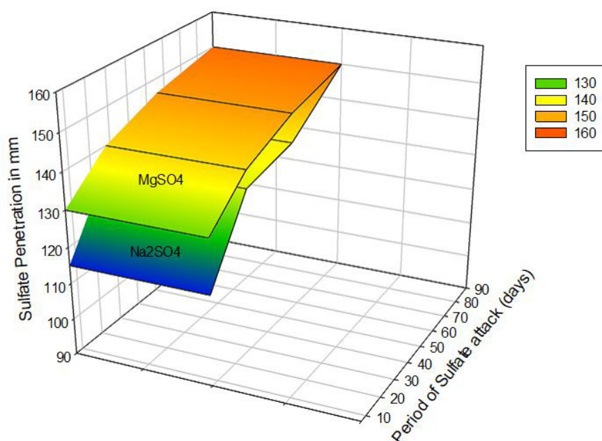
Figure 16: Penetration Depth for Concrete Immersed in \text{Na}_2\text{SO}_4 and \text{MgSO}_4 Moderate and Severe Solutions
