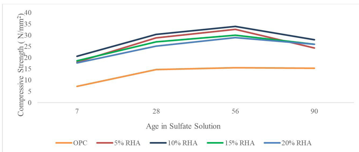
Figure 5: Compressive Strength Test Result for Concrete Immersed in \text{MgSO}_4 Severe Solution ((30,000 mg/L concentration)
